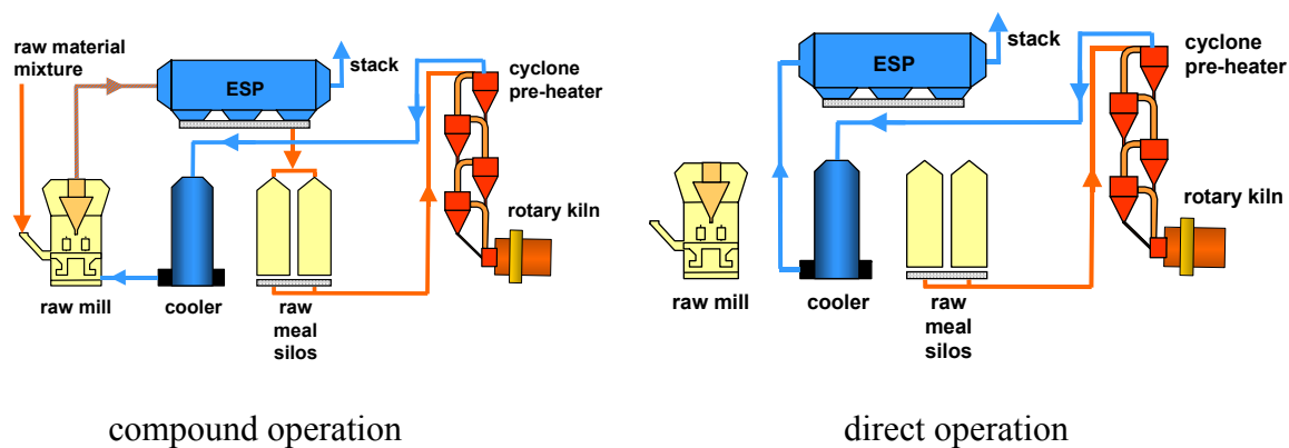
Figure 2: Compound and direct operation in cement production.
