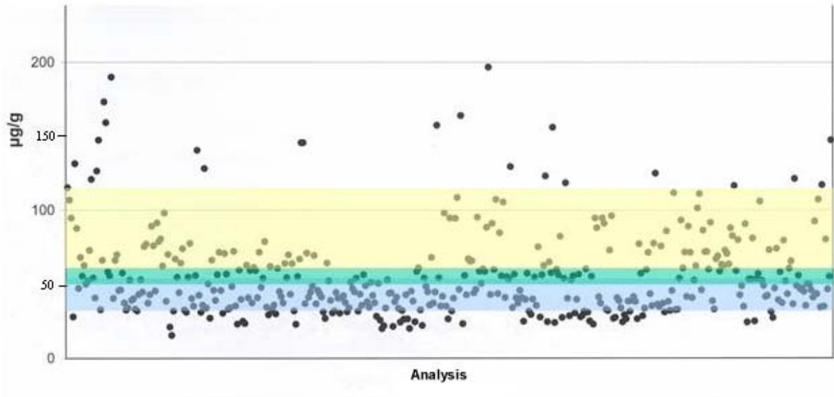
Figure 24: Measured vanadium contents of normal cements [VDZ, 2000]. Yellow bar: concentration range in Portland cement calculated by the bottom-up approach. Blue bar: concentration range in blastfurnace cement calculated by the bottom-up approach. Green bar: overlapping concentration ranges of Portland and blastfurnace cements.
