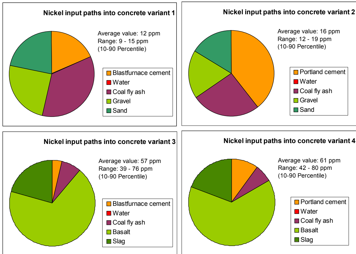
Figure 31: Mean nickel concentrations and concentration ranges in the four concrete variants. Relative shares of the individual input materials in the total nickel concentration of concrete.
