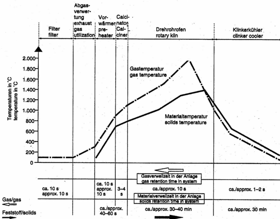
Figure A1: Gas and solids temperature profiles in a cyclone preheater kiln system [VDI 2094, 2003].
