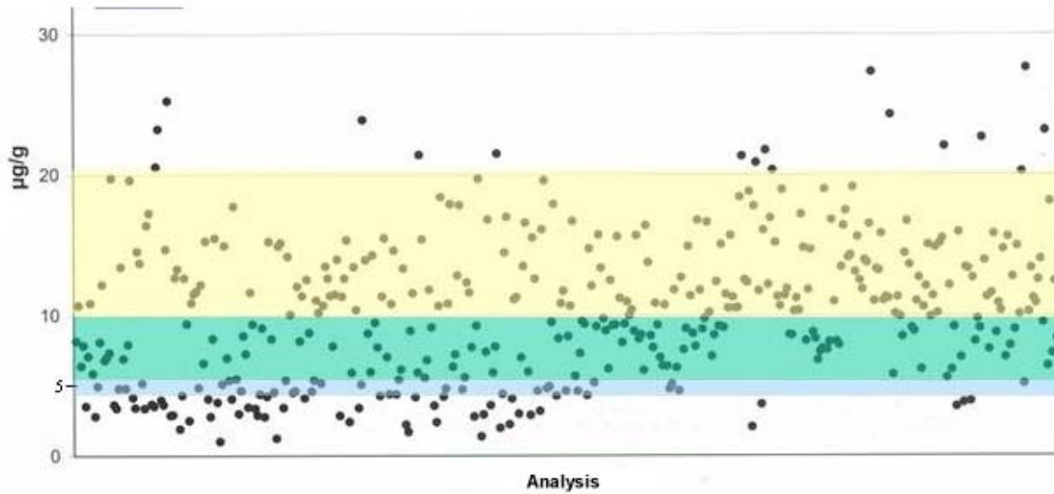
Figure 18: Measured cobalt contents of normal cements [VDZ, 2000]. Yellow bar: concentration range in Portland cement calculated by the bottom-up approach. Blue bar: concentration range in blastfurnace cement calculated by the bottom-up approach. Green bar: overlapping concentration ranges of Portland and blastfurnace cements.
