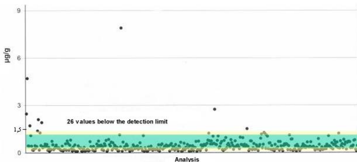
Figure 17: Measured cadmium contents of normal cements [VDZ, 2000]. Yellow bar: concentration range in Portland cement calculated by the bottom-up approach. Blue bar: concentration range in blastfurnace cement calculated by the bottom-up approach. Green bar: overlapping concentration ranges of Portland and blastfurnace cements.
