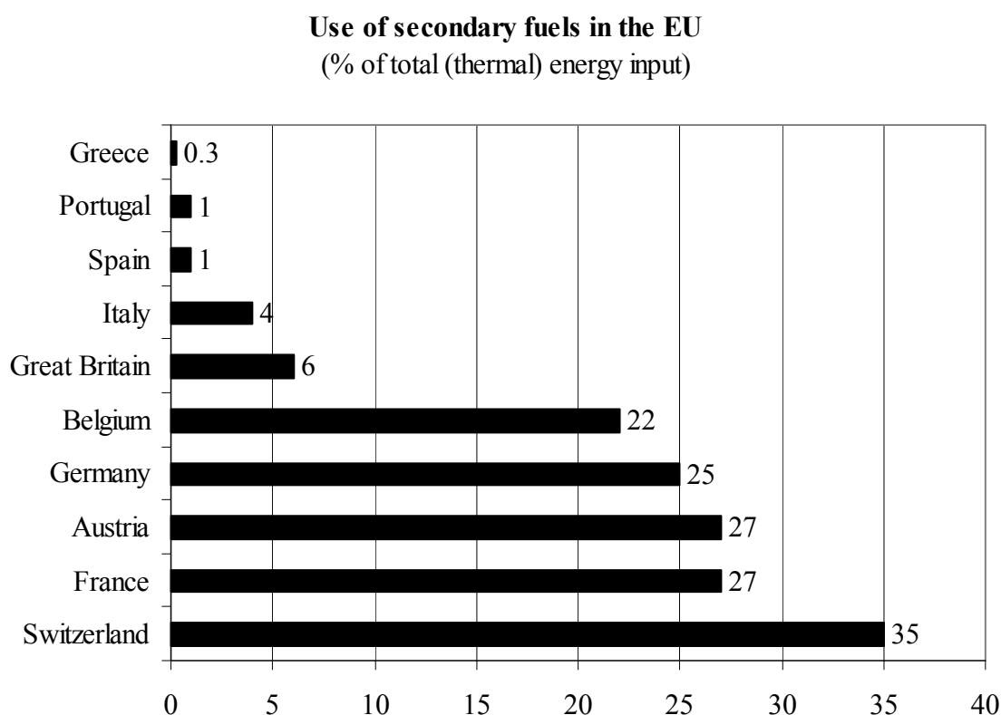
Figure 38: Shares of the secondary fuels used in the total (thermal) energy input in various countries in 2000 [Oficemen, 2003].
