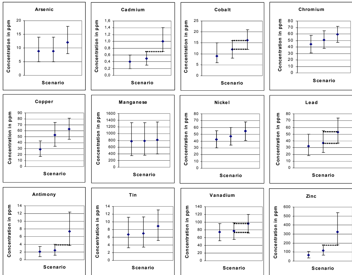
Figure 26: Average trace element concentrations and their ranges in Portland cement in scenarios A (left), B (middle), and C (right).
