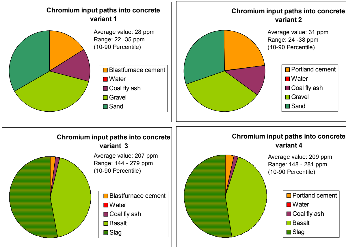
Figure 30: Mean chromium concentrations and concentration ranges in the four concrete variants. Relative shares of the individual input materials in the total chromium concentration of concrete.
