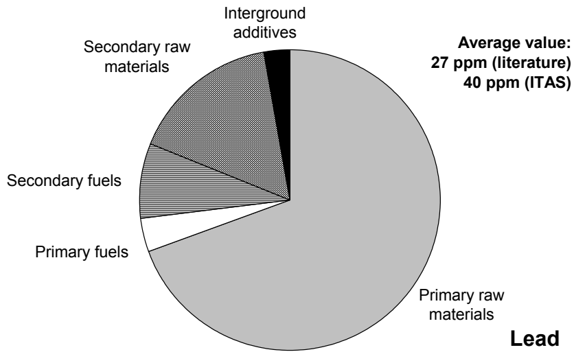
Figure 10: Category IV; relative shares of the individual input paths in the lead content of Portland cement.
