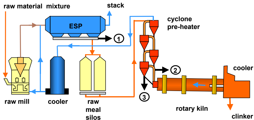
Figure 3: Schematic representation of bypass variants (1: dust bypass, 2: hot gas bypass, 3: hot meal bypass).
