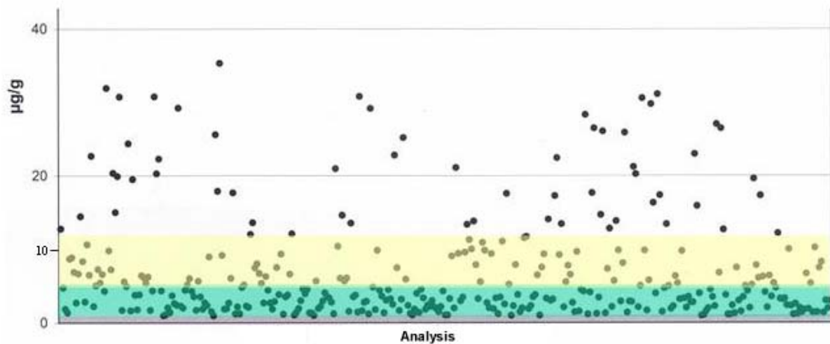
Figure 23: Measured antimony contents of normal cements [VDZ, 2000]. Yellow bar: concentration range in Portland cement calculated by the bottom-up approach. Blue bar: concentration range in blastfurnace cement calculated by the bottom-up approach. Green bar: overlapping concentration ranges of Portland and blastfurnace cements.
