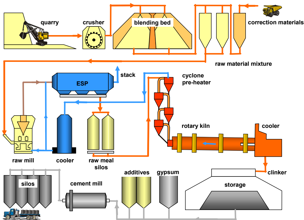
Figure 1: Schematic representation of cement production.
