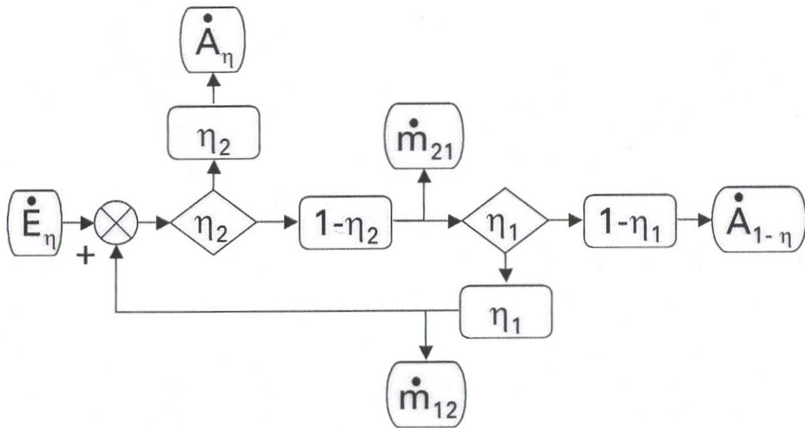
Figure 47: Two-stage model system used for the derivation of transfer factors [Locher, 1999].
