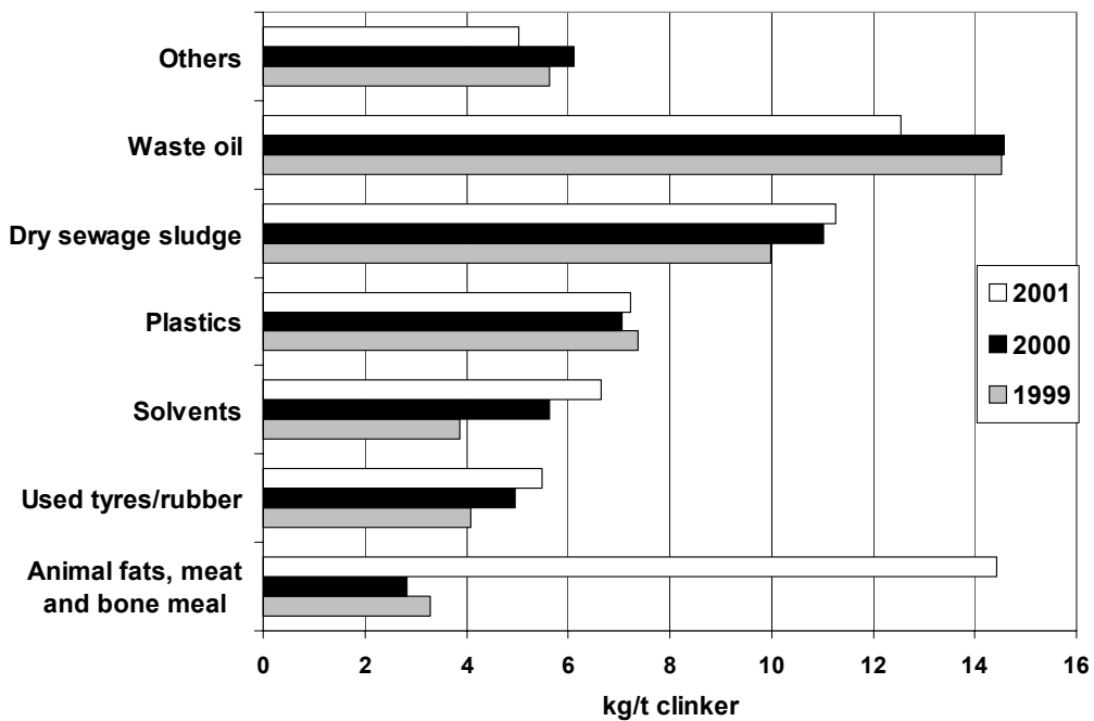
Figure 41: Estimated use of secondary fuels in Switzerland [Cemsuisse, 2000, 2001]. Data are given in kg/t clinker.
