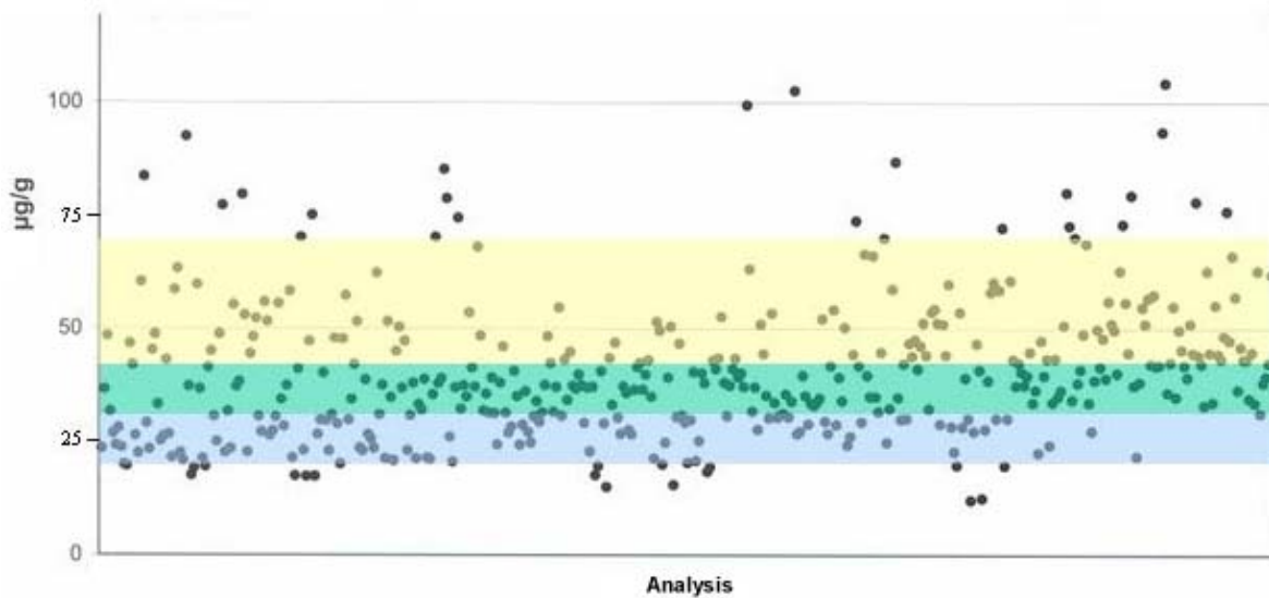
Figure 19: Measured chromium contents of normal cements [VDZ, 2000]. Yellow bar: concentration range in Portland cement calculated by the bottom-up approach. Blue bar: concentration range in blastfurnace cement calculated by the bottom-up approach. Green bar: overlapping concentration ranges of Portland and blastfurnace cements.
