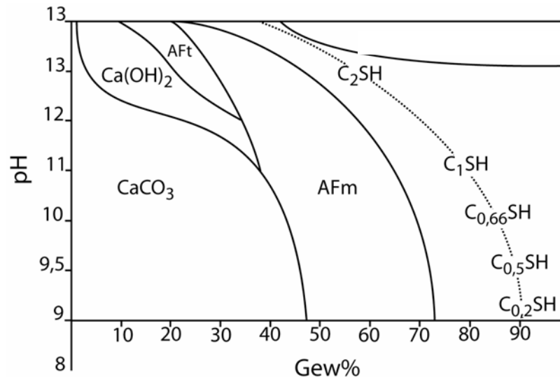
Figure 36: Phase inventory of Portland cement pastes during diffusion-controlled acid weathering, plotted as a function of the pH value.
