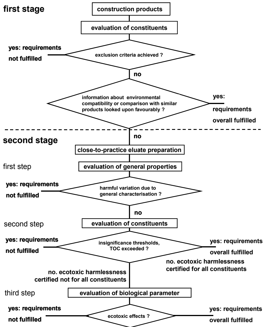
Figure 45: Flow chart for the assessment of construction products with regard to soil and groundwater protection [DIBt, 2000].
