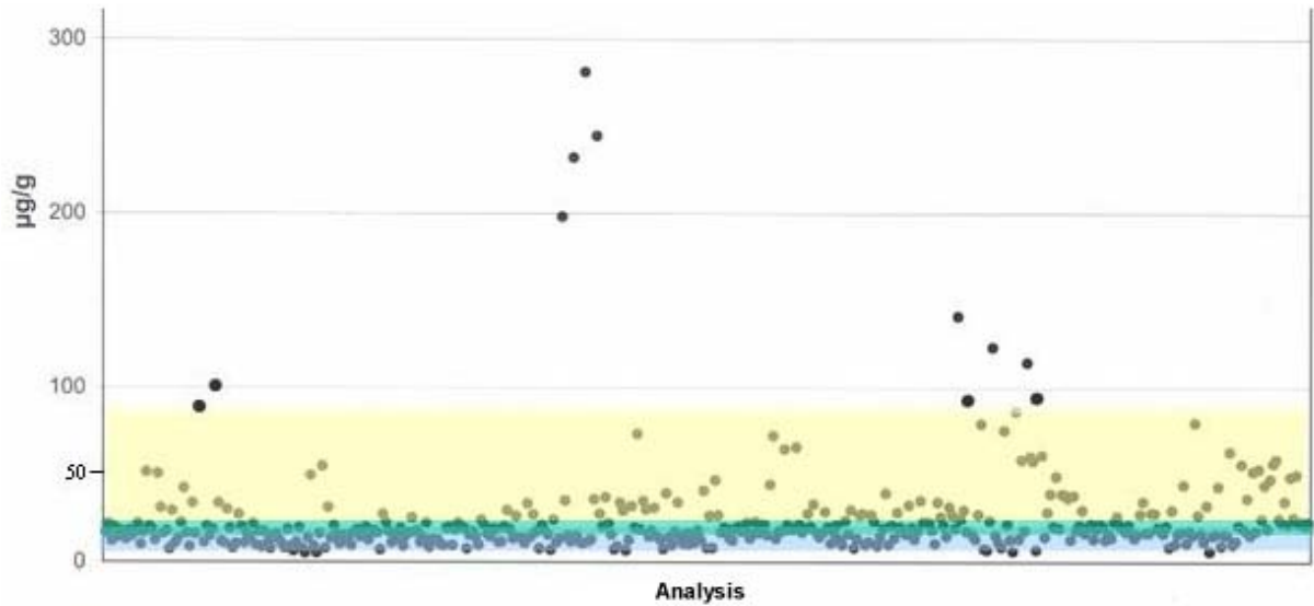
Figure 20: Measured copper contents of normal cements [VDZ, 2000]. Yellow bar: concentration range in Portland cement calculated by the bottom-up approach. Blue bar: concentration range in blastfurnace cement calculated by the bottom-up approach. Green bar: overlapping concentration ranges of Portland and blastfurnace cements.
