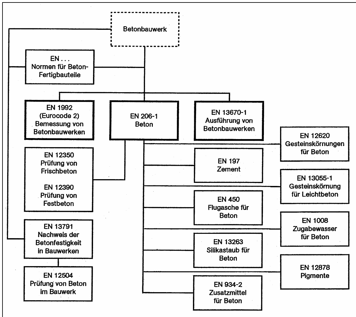
Figure 43: Relations between the EN 206-1 standard and other standards [DIN EN 206-1].
