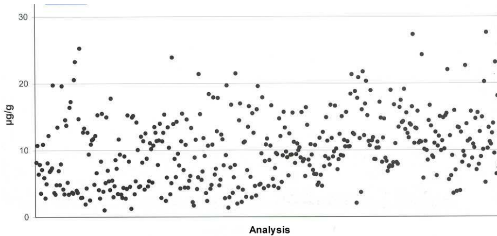
Figure 12: Cobalt concentrations measured in the normal cements [VDZ, 2000].
