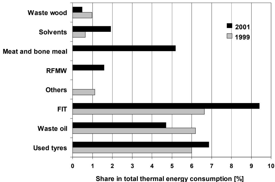
Figure 37: Share of individual secondary fuels in the total thermal energy consumption 1999 and 2001. RFMW: reprocessed fractions of municipal wastes, FIT: fractions from industry and trade [VDZ, 2000, 2002].
