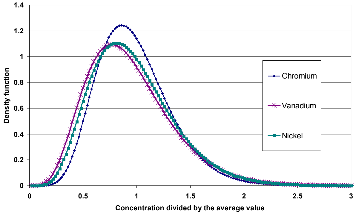
Figure 15: Probability density calculated for concentration values of selected trace elements in normal cements, based on VDZ measurements [VDZ, 2000].
