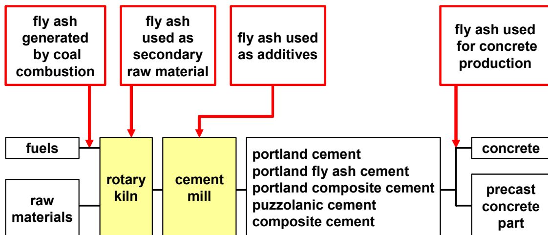
Figure 44: Possible pathway of fly ash from power plants, similar to [Jacobs, 1982].
