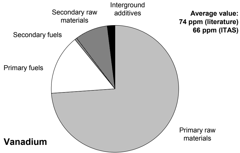
Figure 6: Category II; relative shares of the individual input paths in the vanadium content of Portland cement.
