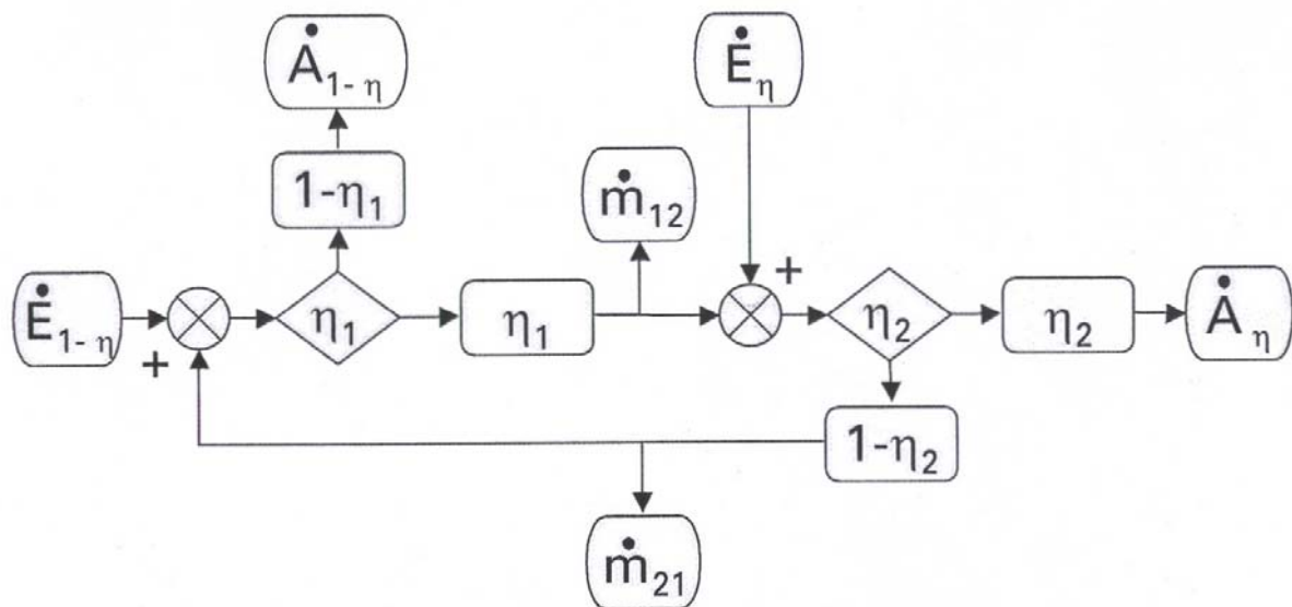
Figure 46: Two-stage model system used for the derivation of emission factors [Locher, 1999].
