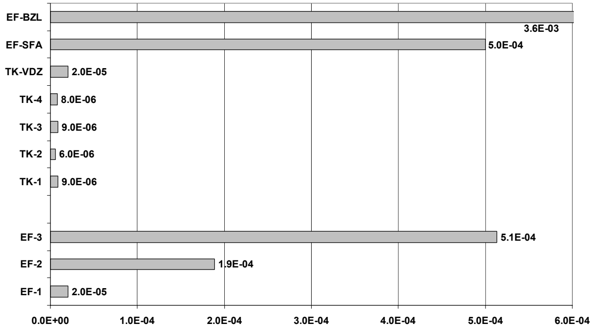
Figure 48: Emission and transfer factors for lead according to [Fehringer et al., 1999], [MURL, 2001].
