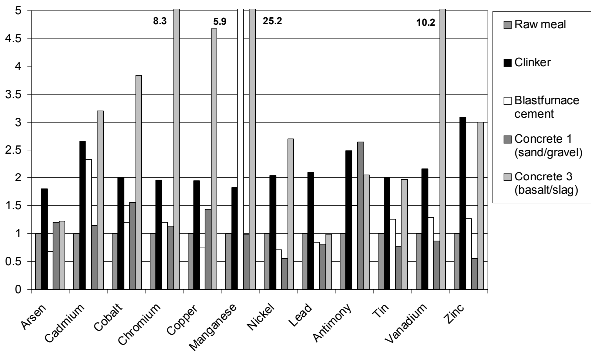
Figure 28: Comparison of the trace element concentrations in concretes from blastfurnace cement with those of raw meal, clinker, and blastfurnace cement. Normalisation to raw meal.
