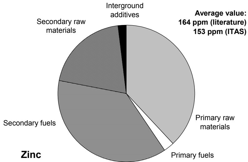
Figure 4: Category I; relative shares of the individual input paths in the zinc content of Portland cement.
