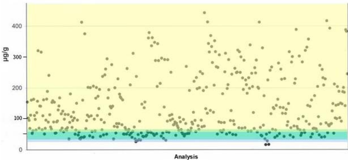
Figure 25: Measured zinc contents of normal cements [VDZ, 2000]. Yellow bar: concentration range in Portland cement calculated by the bottom-up approach. Blue bar: concentration range in blastfurnace cement calculated by the bottom-up approach. Green bar: overlapping concentration ranges of Portland and blastfurnace cements.
