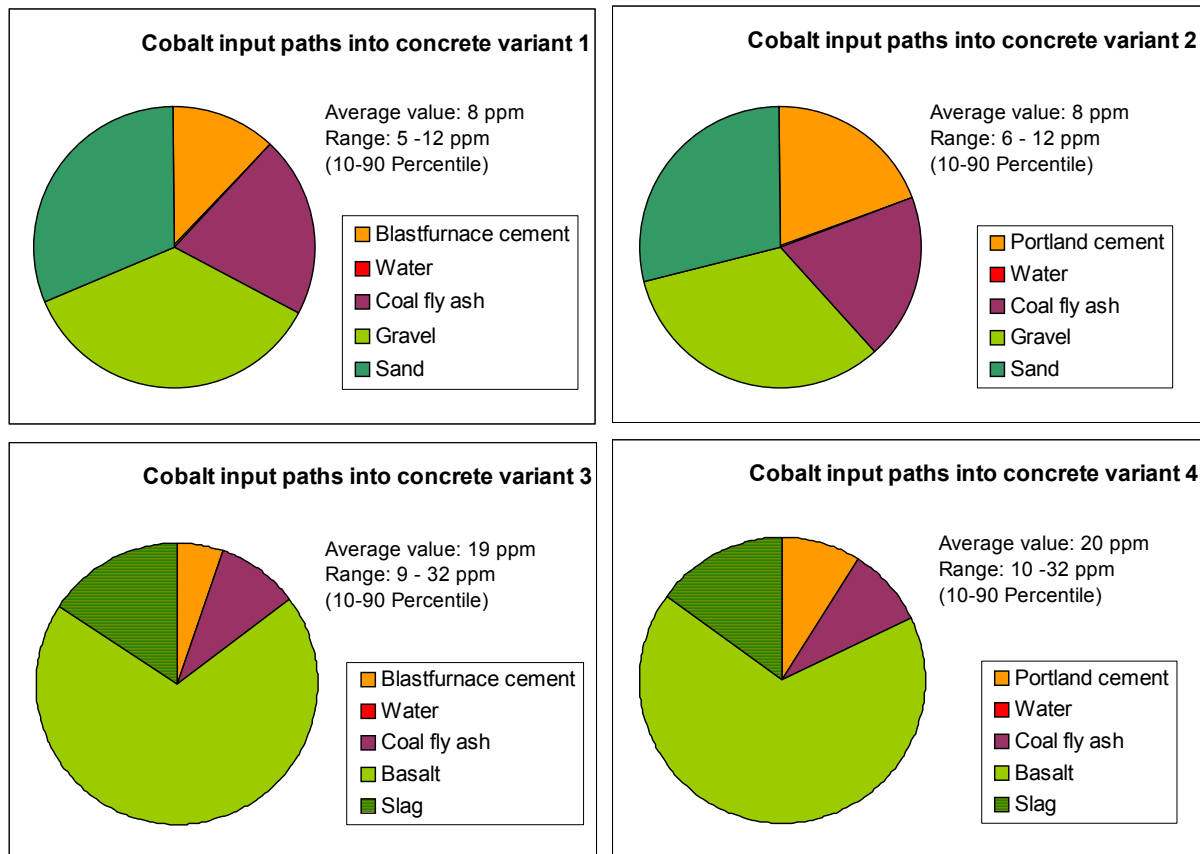
Figure 29: Mean cobalt concentrations and concentration ranges in the four concrete variants. Relative shares of the individual input materials in the total cobalt concentration of concrete.
