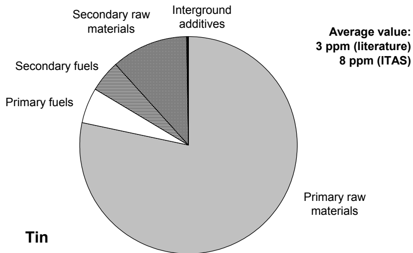
Figure 11: Category IV; relative shares of the individual input paths in the tin content of Portland cement.
