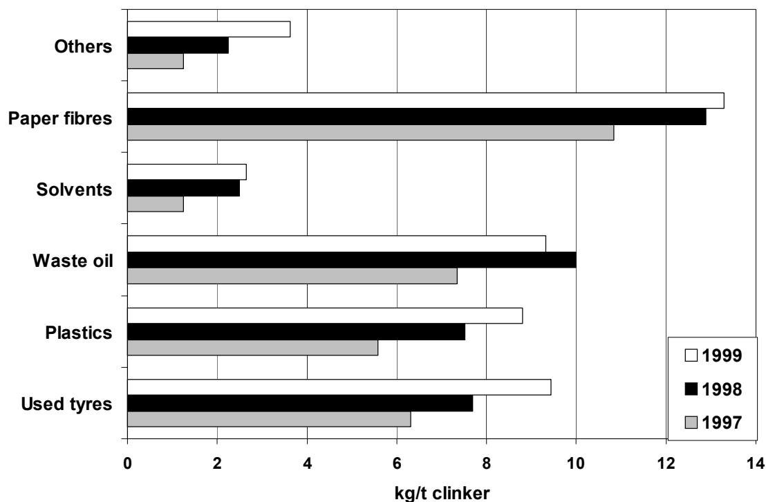
Figure 39: Specific amounts of waste fuels used in Austria [Hackl and Mauschwitz, 2001].
