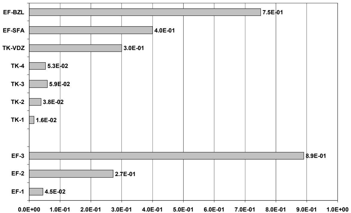
Figure 49: Emission and transfer factors for mercury according to [Fehringer et al., 1999], [MURL, 2001].
