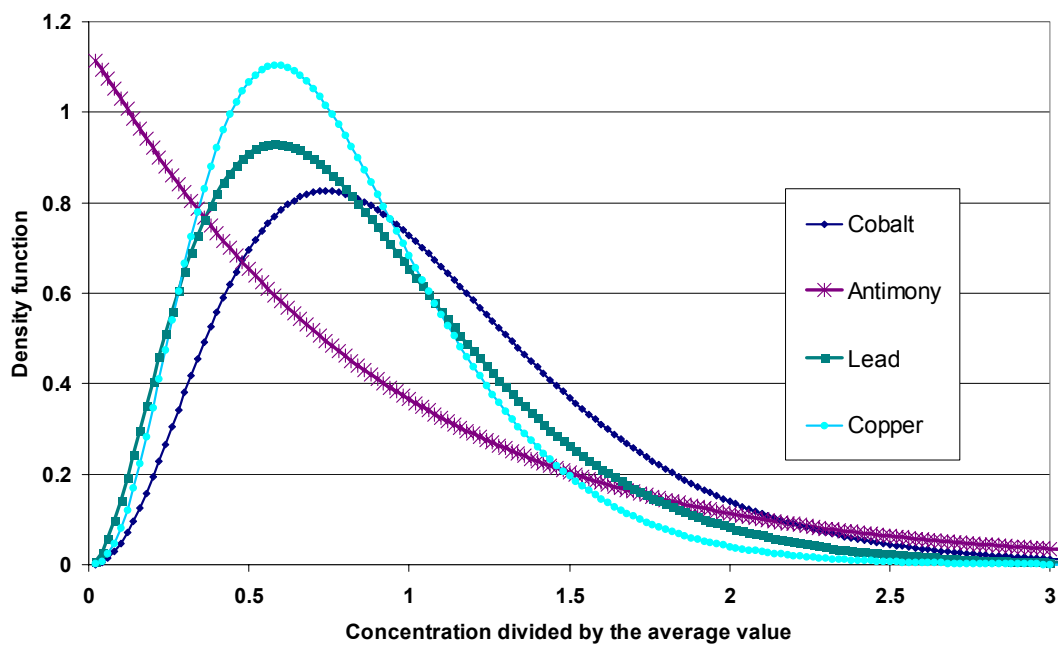
Figure 16: Probability density calculated for concentration values of selected trace elements in normal cements, based on VDZ measurements [VDZ, 2000].
