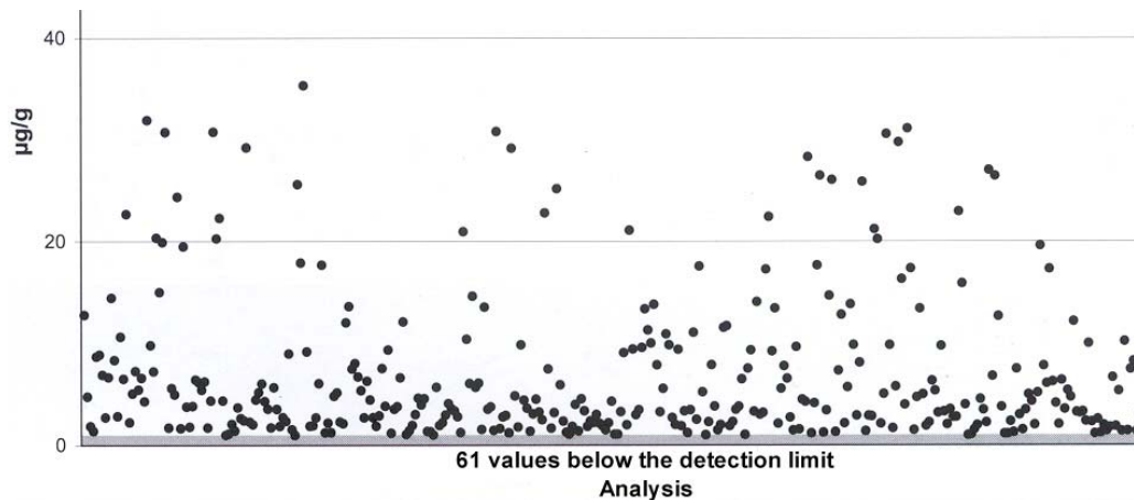
Figure 13: Antimony concentration measured in the normal cements [VDZ, 2000].
