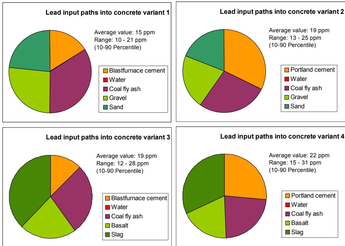
Figure 32: Mean lead concentrations and concentration ranges in the four concrete variants. Relative shares of the individual input materials in the total lead concentration of concrete.
