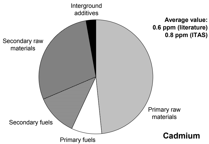
Figure 5: Category I; relative shares of the individual input paths in the cadmium content of Portland cement.
