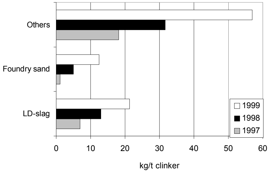
Figure 40: Use of secondary raw materials in Austria [Hackl and Mauschwitz, 2001]. LD slag: steel works slag resulting from the Linz-Donawitz process.
