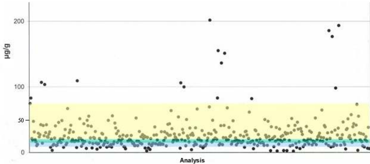
Figure 22: Measured lead contents of normal cements [VDZ, 2000]. Yellow bar: concentration range in Portland cement calculated by the bottom-up approach. Blue bar: concentration range in blastfurnace cement calculated by the bottom-up approach. Green bar: overlapping concentration ranges of Portland and blastfurnace cements.
