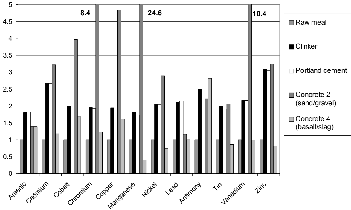
Figure 27: Comparison of the trace element concentrations in concretes from Portland cement with those of raw meal, clinker, and Portland cement. Normalisation to raw meal.
