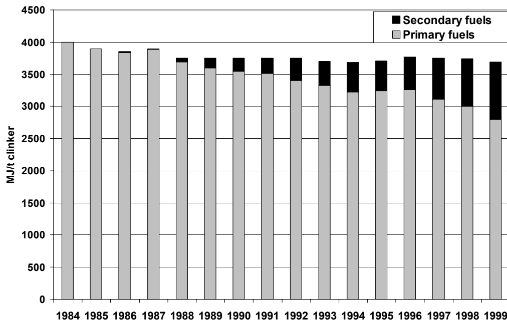
Figure 42: Waste co-combustion in France from 1984 to 1999 [Boyed, 2001].
