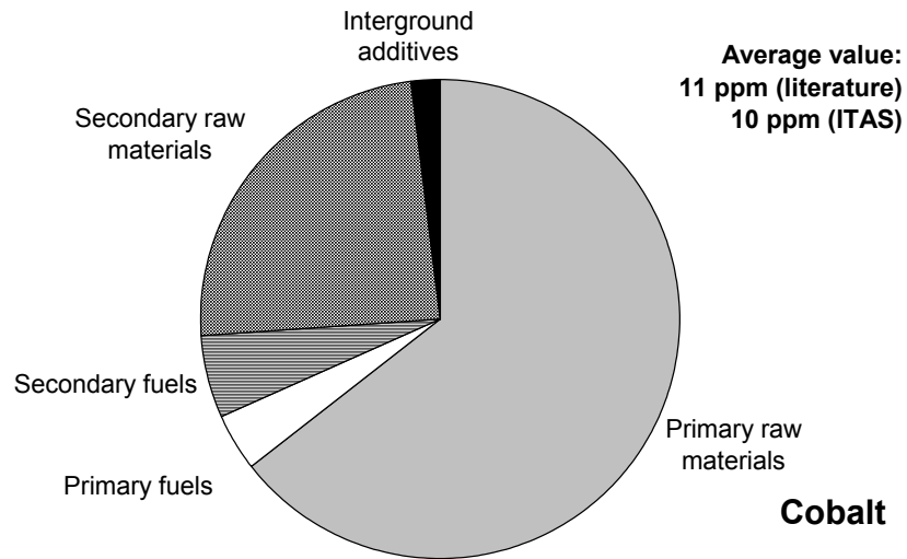
Figure 8: Category III; relative shares of the individual input paths in the cobalt content of Portland cement.
