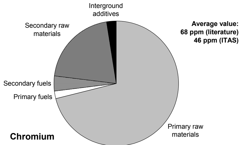
Figure 9: Category III; relative shares of the individual input paths in the chromium content of Portland cement.
