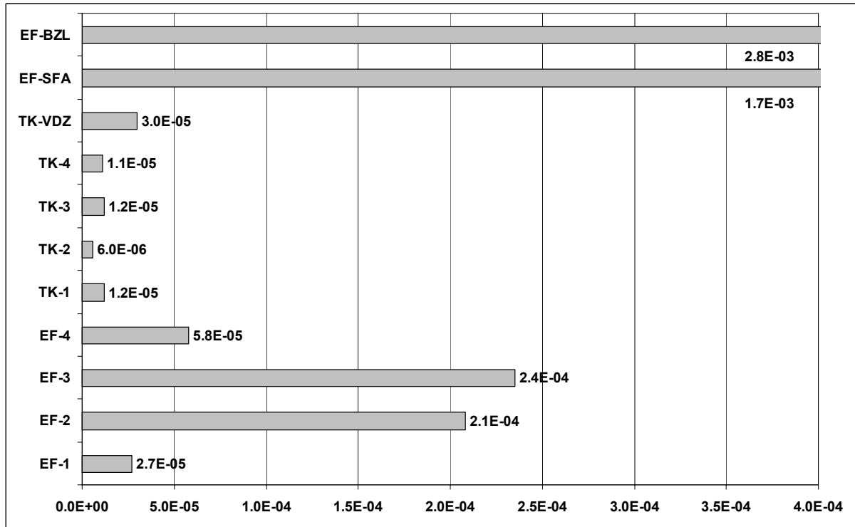
Figure 50: Emission and transfer factors for cadmium according to various sources [Fehring et al., 1999], [MURL, 2001].
