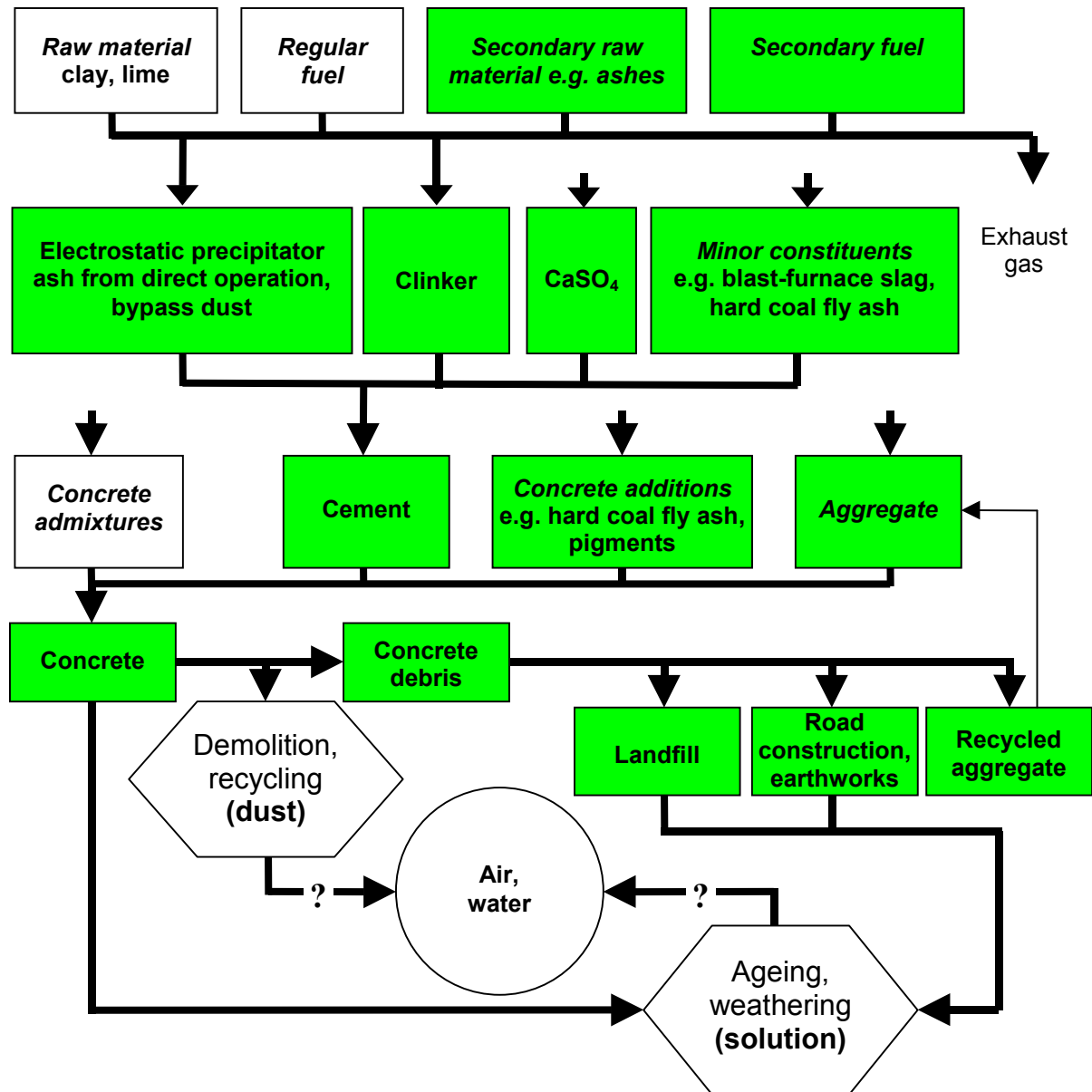
Figure 33 : Origin, transport, and whereabouts of trace elements of a concrete building. Shaded areas might be influenced by the use of waste in cement production.
