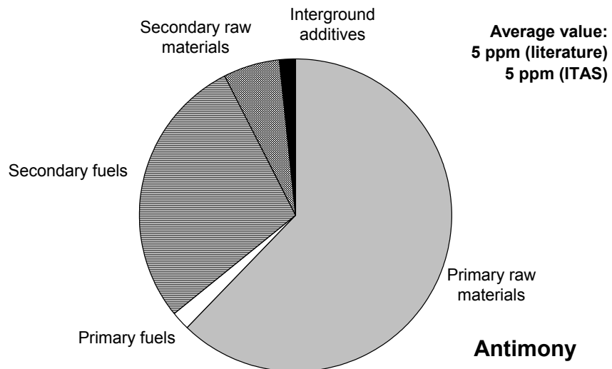
Figure 7: Category II; relative shares of the individual input paths in the antimony content of Portland cement.
