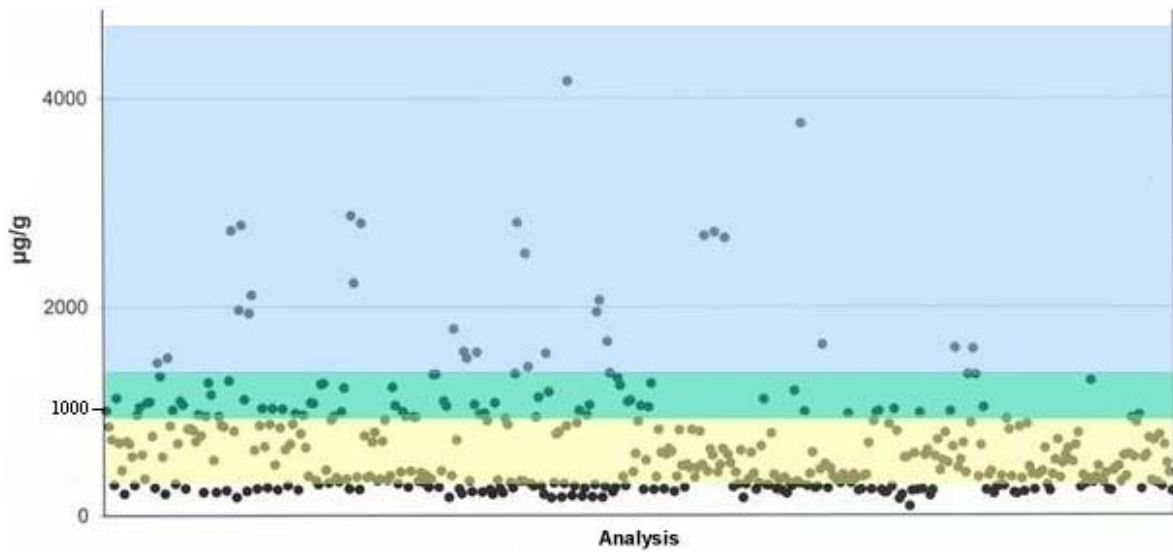
Figure 21: Measured manganese contents of normal cements [VDZ, 2000]. Yellow bar: concentration range in Portland cement calculated by the bottom-up approach. Blue bar: concentration range in blastfurnace cement calculated by the bottom-up approach. Green bar: overlapping concentration ranges of Portland and blastfurnace cements.
